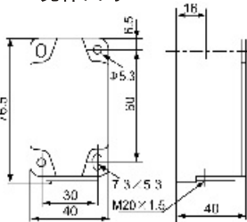
二极窄型3SE3 120 Two-pole narrow housing
